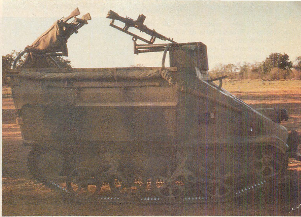
"War on a shoe-string." Rhodesian army is using WW-II Bren gun carrier with four MAG 7.62 machine guns for bush convoy protection.
